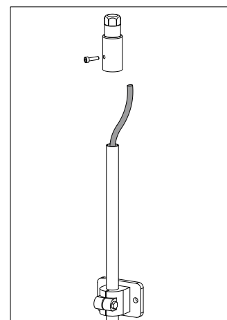
Connection to the wall Indoor/Outdoor - (FK-12 clamp)
