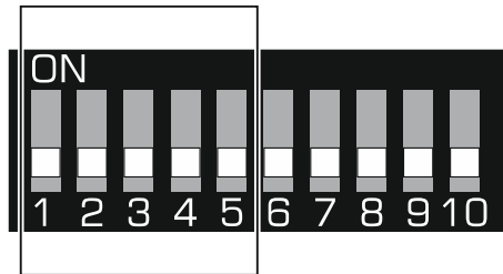
Fig. 4. DIP switches for setting address when the controller is connected to the INTEGRA / INTEGRA Plus control panel.
